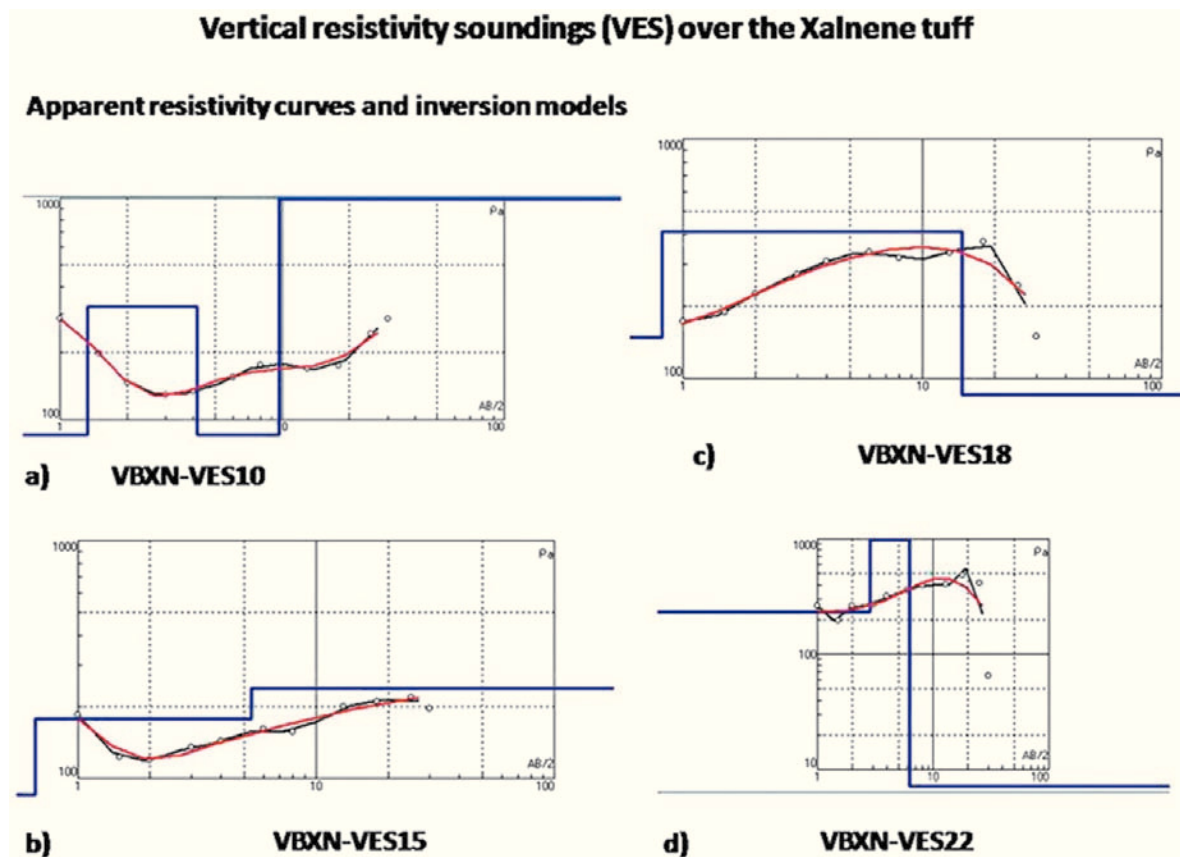
Figure 3. Representative examples of vertical electrical soundings (VES) in Xalnene tuff plain. The inversion models are included in the blue lines.
