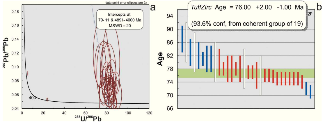
Figure 6. U/Pb zircon data from the granite megablock in the Cañada de Tarachi. a) Concordia curve for the A134-12 sample and b) Weighted mean age graph at 76 Ma.
