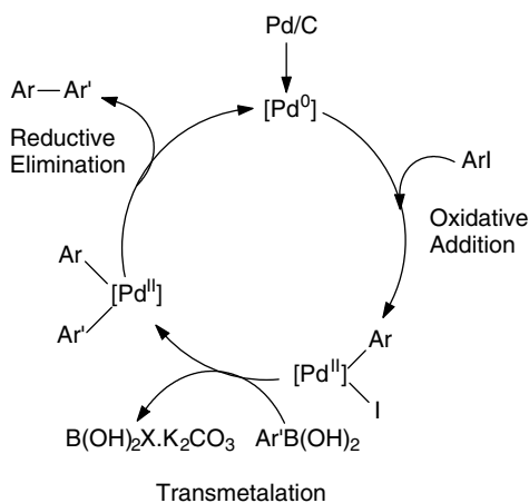
Figure 2 Catalytic cycle of the Suzuki-Miyaura cross-coupling reaction (Oliveira et al., 2015).
