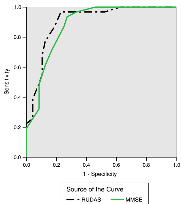
Figure 1 ROC curve for the RUDAS and MMSE in 97 subjects.
