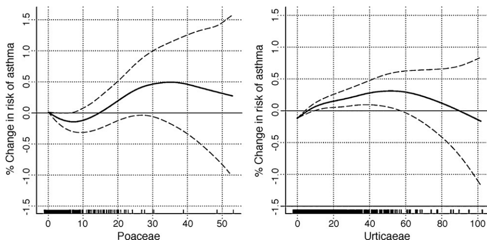
Figure 2 Non-parametric figure of the continuous relative risks values among the daily relationship of aeroallergen pollen types counts (grains/m 3 ) on asthma hospital emergency room visits.
