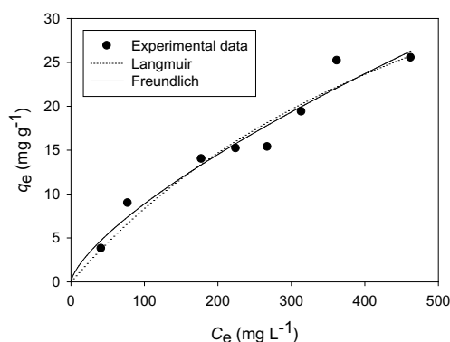
Fig. 1. Experimental and calculated equilibrium data for adsorption of phenol on the aerogel.
