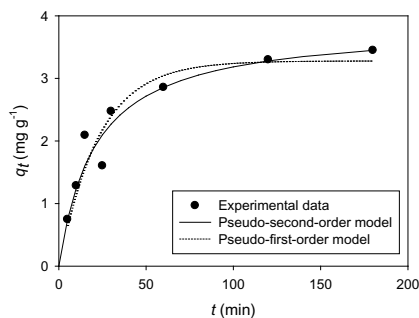
Fig. 3. Adsorption kinetics of phenol on aerogel in a stirred tank ( T = 20^\circ\text{C} , V = 1 \text{ L} , m = 10 \text{ g} , C_0 = 100 \text{ mg/L} ).
