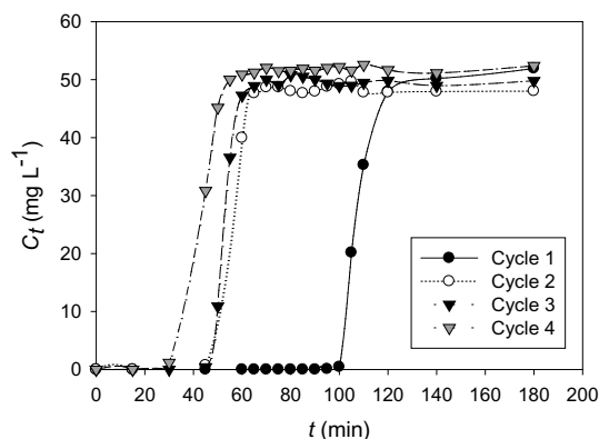
Fig. 4. Breakthrough curves of phenol on aerogel in a fixed bed column ( T = 20^\circ\text{C} , Q = 2 \text{ mL/min} , m = 1.6 \text{ g} , C_0 = 50 \text{ mg/L} ).
