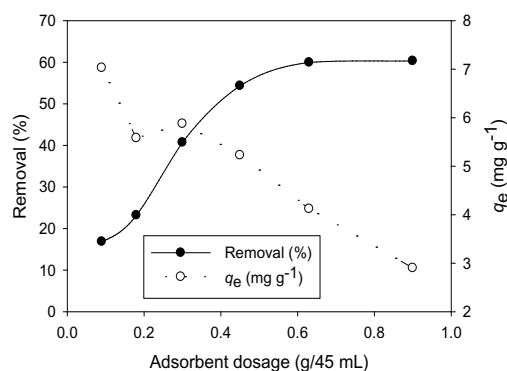
Fig. 2. Effect of adsorbent dosage on phenol removal and adsorbent capacity.
