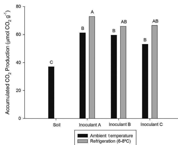
Fig. 8 – The total CO 2 production (μmol CO 2 g -1 ) from gasoline-contaminated soil after application of the inoculants stored at different temperatures. The treatment means followed by the same letter do not differ at 5% probability by Tukey's test. Inoculant A (A); B (B); and C (C). Inoculants A and B received nutrients plus water and gasoline in distinct times for the enrichment of hydrocarbonoclastic populations. Inoculant C refers to MSWC with no gasoline added.
