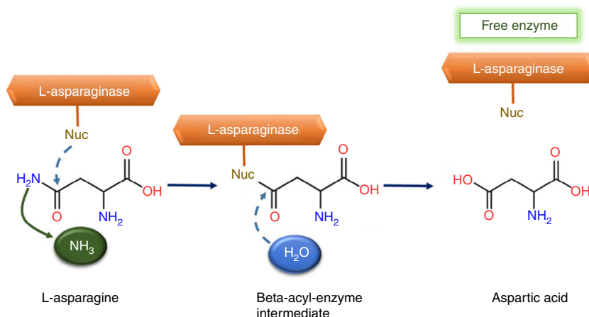
Fig. 1 – General mechanism of L-asparaginase reaction catalyzed. Dashed arrow shows nucleophilic attack. Source: Based on Hill (1967) 9 cited by El-Bessoumy et al. (2004), 10 and Shrivastava et al. (2016). 11
