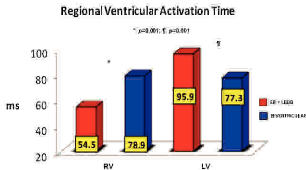
Figure 2 - Comparison of regional RV and regional LV activation times during sinus rhythm and biven-tricular pacing.
