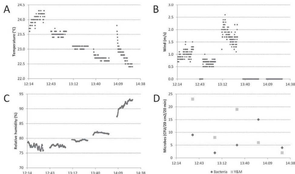
Figure 2. Atmospheric conditions in The Great Cavern of Santo Tomás from the cave entrance towards the cave interior (5, 15, 25, 100, 120 m, deep in the cave, see text for details) on 22 December 2011: A, measured air temperature; B, air inflow; C, relative humidity; D, cultivable airborne bacteria (Bacteria) and yeast and moulds (Y&M) expressed as Colony-Forming-Units CFU/20 cm 2 /20 min.
