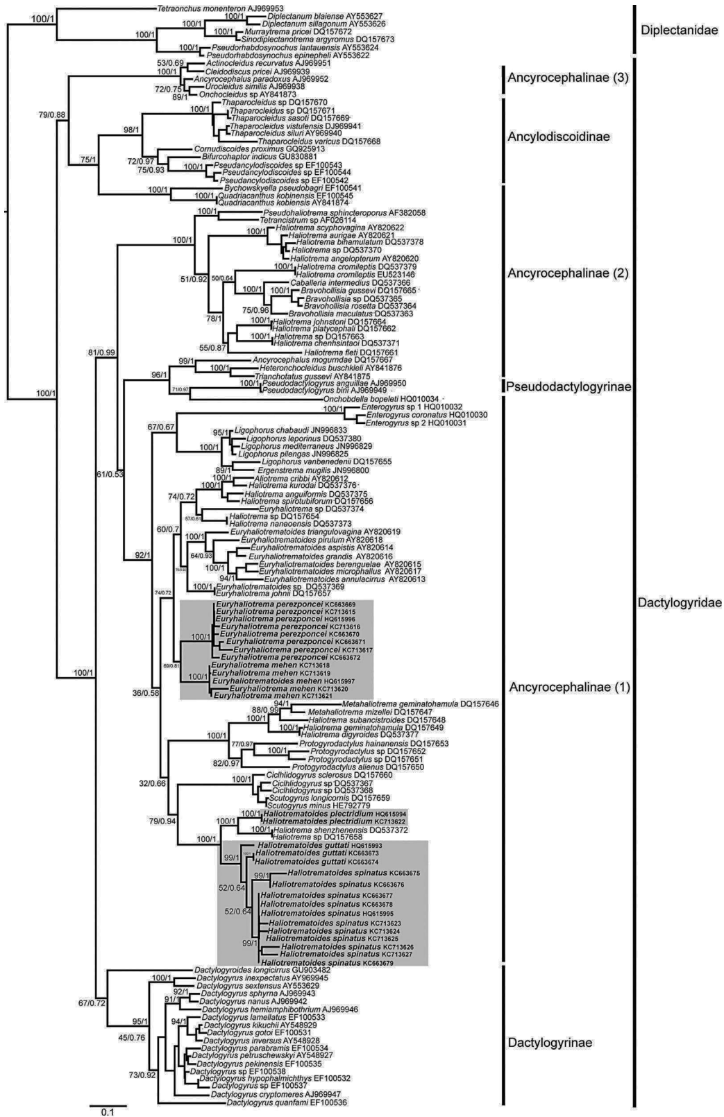
Figure 16. Phylogenetic tree obtained through from maximum likelihood (ML) analysis based on the 28S sequences for selected dactylogyrid species, with some species of diplectanids used as outgroups.
