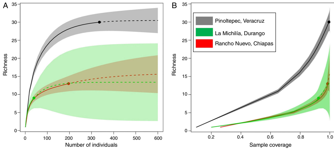
Figure 2. (A) Size-base rarefaction (solid curves) and extrapolation (dash curves) comparing Saturniidae species richness in Pinoltepec, Veracruz (present study), Rancho Nuevo, Chiapas (Beutelspacher & Balcázar, 1998) and La Michilía, Durango (Díaz & Balcázar, 1997); (B) coverage-based rarefaction and extrapolation curve. Shadow areas represent the 95% confidence intervals (bootstrap method with 300 replication).
